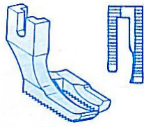
Ref : Walking foot outside U-192 H 1/8" 071.350.730 U-192 J 5/32" 071.350.735 U-192 L 3/16" 071.350.740 U-192 G 7/32" 071.350.745 U-192 K 1/4" 071.350.630 U-192 M 5/16" 071.350.750 U-192 N 3/8" 071.350.755
