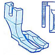
Ref : Walking foot outside U-192 HC 1/8" 071.350.731 U-192 JC 5/32" 071.350.736 U-192 LC 3/16" 071.350.741 U-192 GC 7/32" 071.350.656 U-192 KC 1/4" 071.350.656 U-192 MC 5/16" 071.350.751 U-192 NC 3/8" 071.350.756
