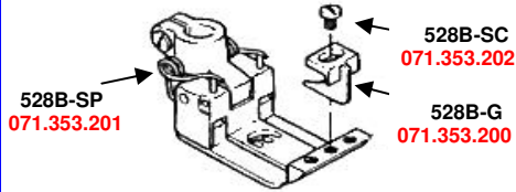
Ref : 528 B Special cover seaming foot
